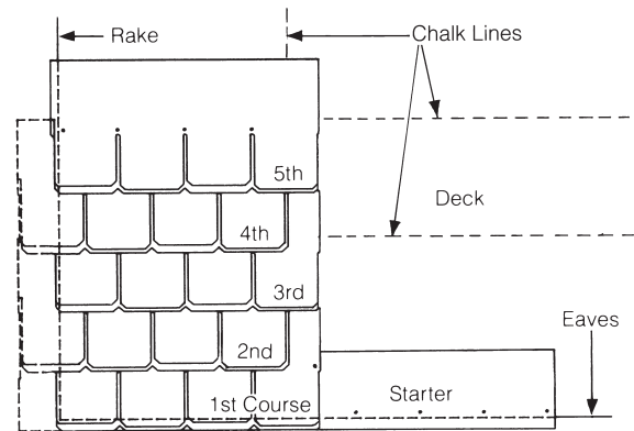
Figure 17-6: Vertical Racking Method.
