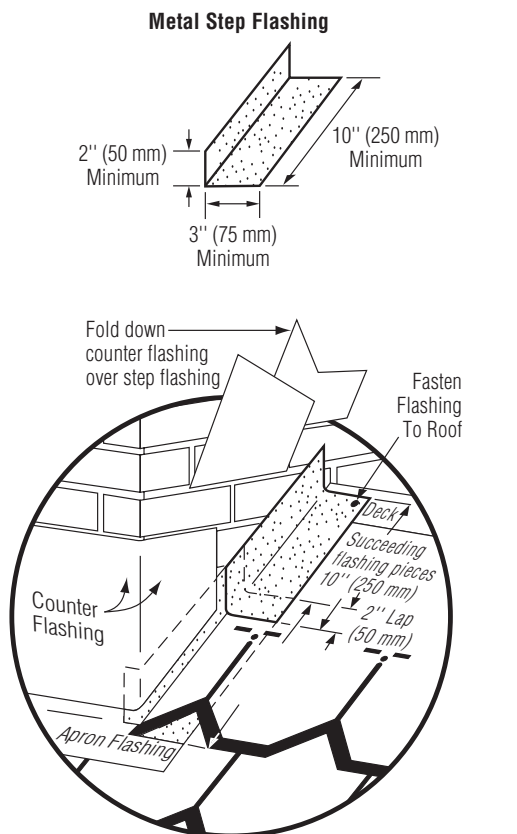
Figure 17-14: Metal step flashing for Carriage House.
