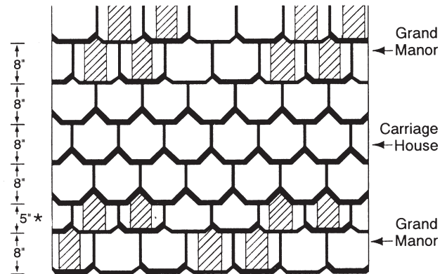
Figure 17-21: Blending Carriage House with Grand Manor.
