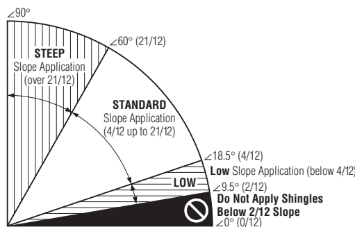
Figure 17-2: Slope definitions.
